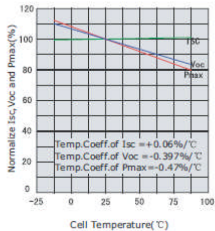
Temperature dependence of Isc, Voc and Pmax
